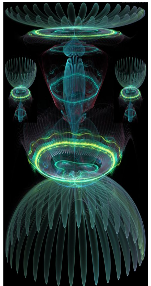
Fig. 7.5. Weaving the first and second subcont-antisubcont currents, circulating between the core of the «stars» and core of the «planet»
