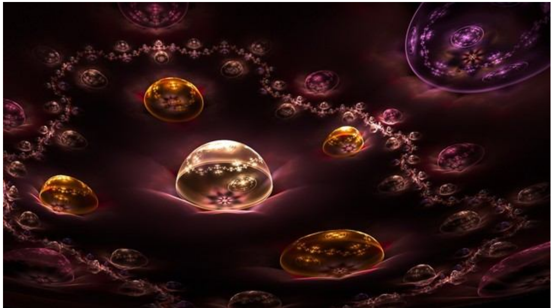
Fig. 2.4. Fractal illustration of the results of probing the location of the «star» (and /or «planet») with rays of light from the wavelength range \Delta\lambda = 10^6 - 10^7 cm. In this wavelength range of the «star» and «planet» (more precisely, the landscapes \lambda_{1,3} -vacuum) look like a star system consisting of single spherical vacuum formations
