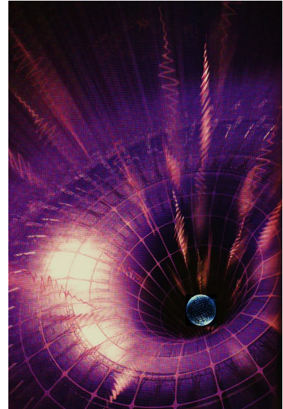
Fig. 2.5. Illustration of the length of \lambda_{6,7} -vacuum in the vicinity of the naked core "stars" or core "planets»
