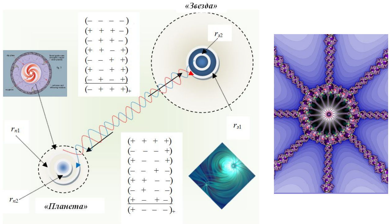
Fig. 7.5. Weaving the first and second subcont-antisubcont currents, circulating between the core of the «stars» and core of the «planet»
