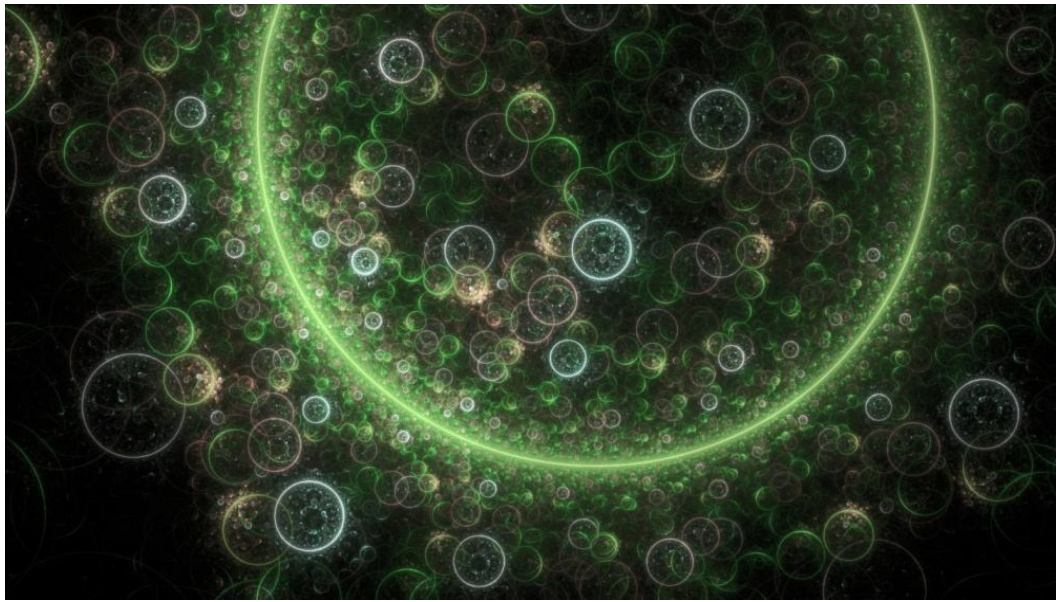
Fig. 2.2. Fractal illustration of the results of probing the location of the «star» (and /or «planet») with rays of light from the wavelength range \Delta\lambda = 10^{-5} - 10^{-6} cm. In this wavelength range of the «star» and «planet» (more precisely, the landscapes \lambda_{-5, -6} -vacuum) look consisting of of biological «cells», «bacteria», «viruses» and other «microorganisms»
