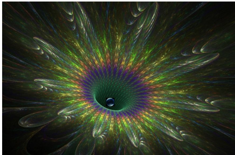
Fig. 6.4. Fractal illustration of a opposite subcont - antisubcont currents affluent and flowing through the intertwined spirals to/from the core of the «star» («planet»). At each point of this vacuum region, the acceleration of the affluent subcont - antisubcont currents is slightly higher than the acceleration of the flowing subcont - antisubcont currents. Therefore, any body that falls into this region of vacuum extent is, on average, attracted to the core of a «star» (or «planet») with uncompensated acceleration (6.12) [or (6.24)]
