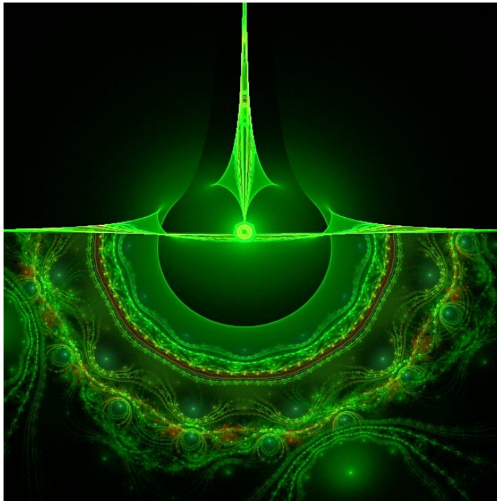
Fig. 6.4. Fractal illustration of intertwined subcont - antisubcont currents flowing in and out of double spirals to / from the rotating core of a «star» (or «planet»)
