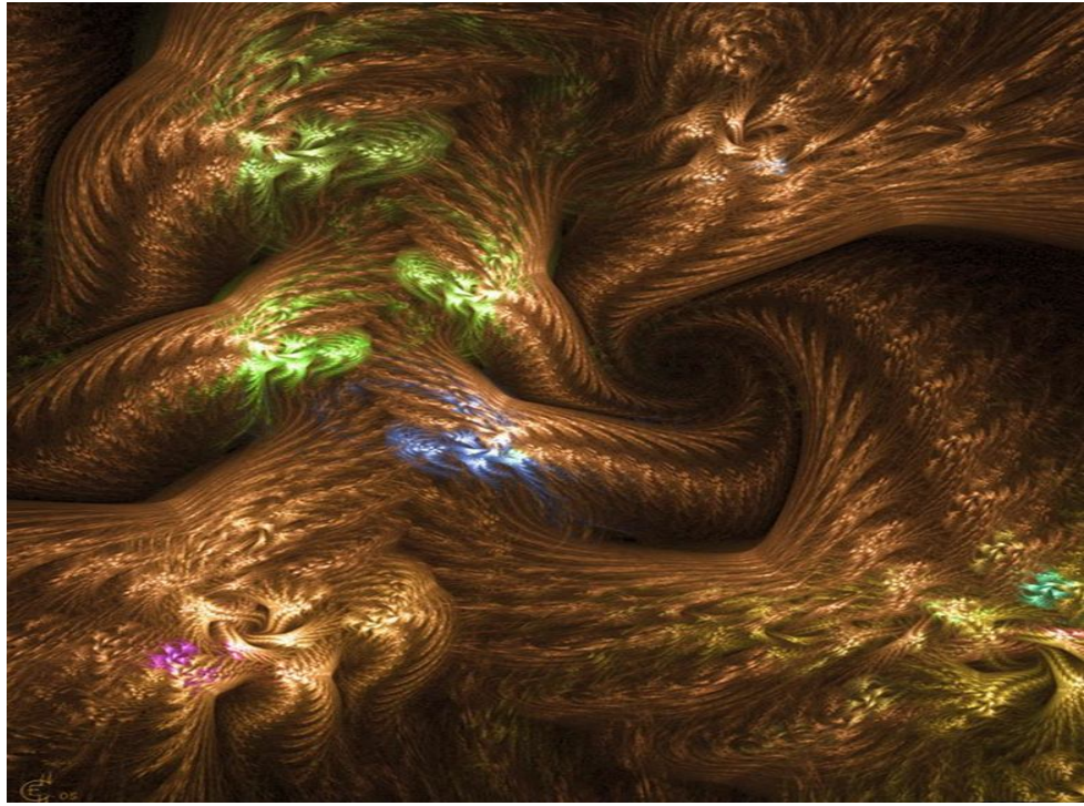
Fig. 6.4. Fractal illustration of intertwined subcont - antisubcont currents flowing in and out of double spirals to / from the rotating core of a «star» (or «planet»)
