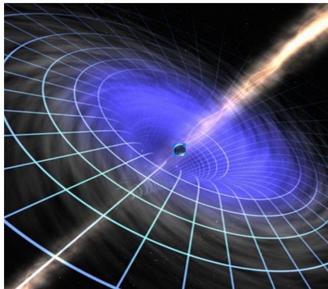
Fig. 2.6. The contours of the metric-dynamic structures naked (transparent) «stars» (or naked «planet»), i.e. a curved landscape area of \lambda_{6,7} -vacuum in the area of the core of macroscopic vacuum formation, which formally «eliminated» all the small «particle», «electrons», «atoms», «molecules», «bacteria» etc. (by means of sensing long wavelength radio waves)
