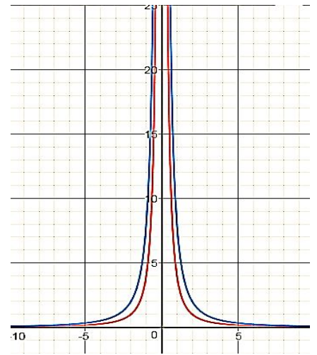
Fig. 6.1. The blue (upper) line a_1/r^2 shows the acceleration of the flowing stream, and the red (lower) line a_2/r^2 shows the deceleration of the flowing stream depending on the distance to the cent of the «star» (or «planet»). In this case, a_1 > a_2 , and the resulting acceleration (a_1 - a_2)/r^2 is relatively small and always directed towards the core of the «star» (or «planet»)
