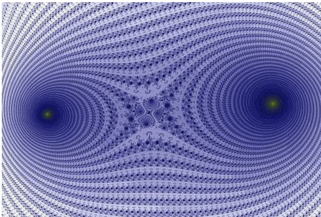
Fig. 7.4. Fractal illustration of the complex interweaving of the first and second subcont-antisubcont currents around the cores of the «stars» and core of the «planet»
