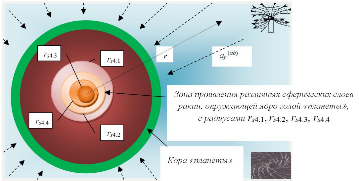
Fig. 6.2. Various spherical layers of rakya surrounding the core of a naked «star» (or «planet»), with r_{s4.1} , r_{s4.2} , r_{s4.3} , r_{s4.4}
