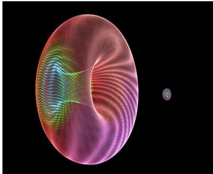
Fig. 5.5. Illustration of the comparative dimensions of aquatic «neutrino» and electronic «neutrino», the radius of the neck which differ by 7 orders of magnitude
