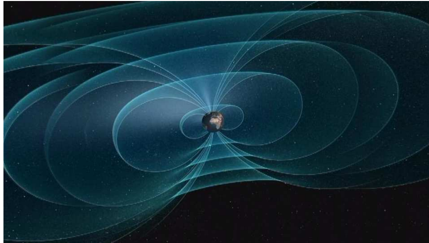
Fig. 8.2. Illustration of a toroidal-helical field of vacuum induction (i.e., magnetic field) induced around a moving and rotating planet (or star) (art. http://static.euronews.com )
