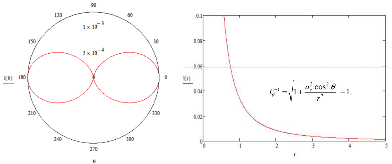
Fig. 3.2. Function graphs (3.7) for r = 10 , a_e = 0.5 , \theta = 10
