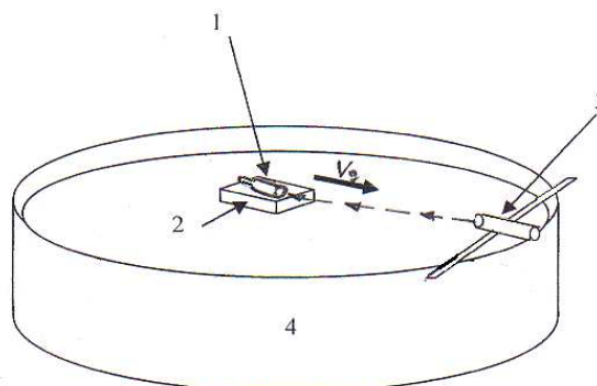
Fig. 5.1. The Volkov impact effect is the movement of the ampoule with magnetized water in the direction of the source of red light (i.e. laser pointers):
