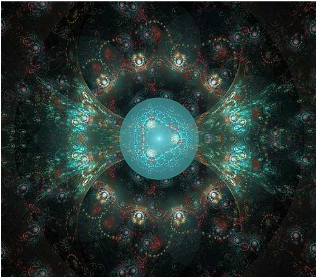
Fig. 7.2. Illustration of the core and outer shell of the resting «proton»
