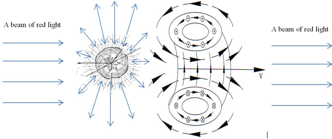
Fig. 5.4. Vacuum toroidal-helical vortex flies from the water cluster with a characteristic size \sim 5 \cdot 10^{-6} \text{ cm}
