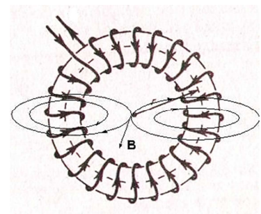
Fig. 5.6. Toroidal magnetic field of a toroidal coil with a direct current
