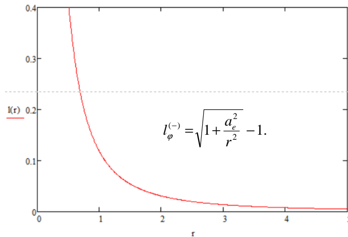
Fig. 3.3. The graph of the function (3.8) with a_e = 0.5 . The calculations are performed using the MathCad software
