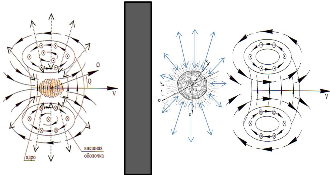
Fig. 4.1. Moving «electron», faced with a solid obstacle, is divided into a resting «electron» and a separate toroidal-helical vortex (i.e. the initial state of the electronic «neutrino»), which continues to move at a speed V_z
