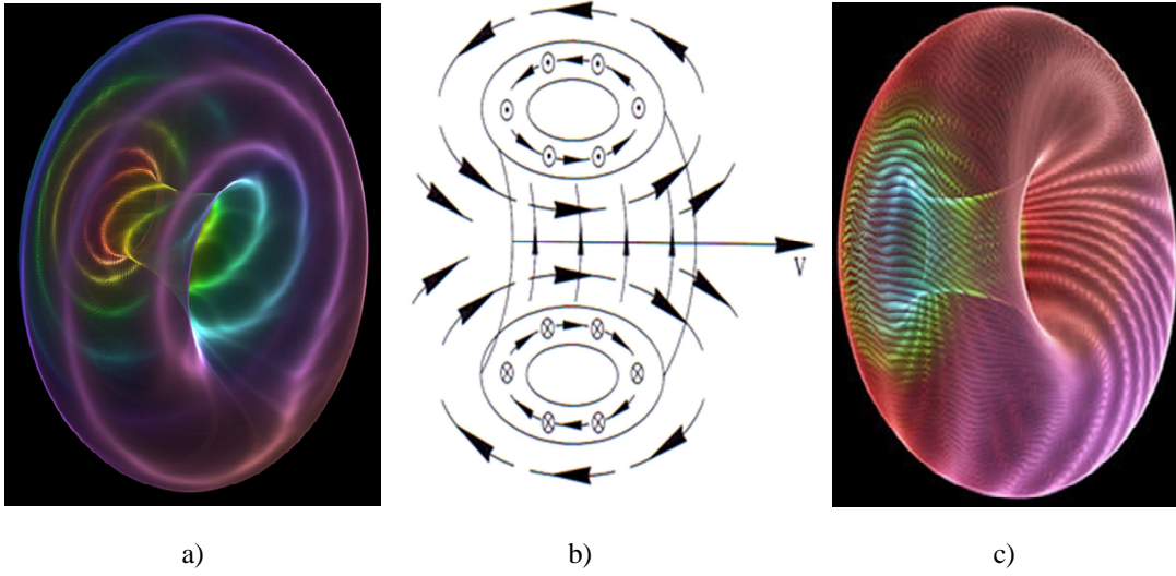
Fig. 4.2. Illustration of the dynamics of a \times b -subcont toroidal-helical vortex, which is called an electronic «neutrino» in the framework of the Alsigna
