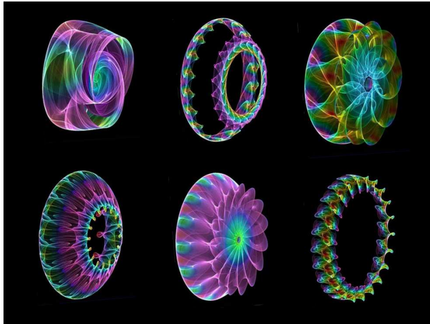
Fig. 6.1. Fractal illustration of different possible configurations of the averaged excited states of «neutrinos»
