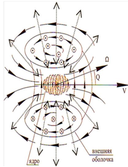
Fig. 1.1. Laminar and turbulent (toroidal-helical) a \times b -subcont accelerated currents in the outer shell of a moving «electron»
