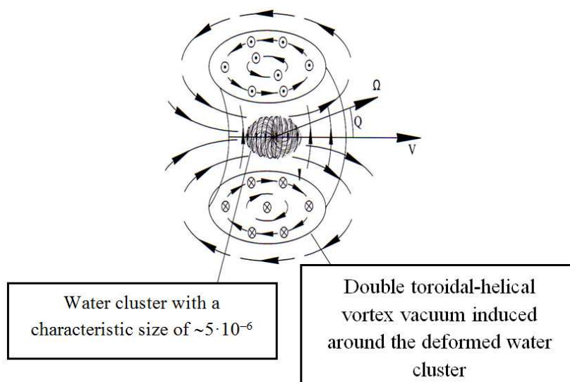
Fig. 5.3. Rotational movement of the vacuum around the deformed water cluster
