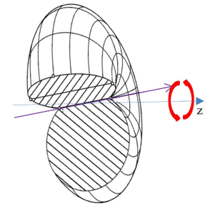
Fig. 6.2. Illustration of the precession of the rotation axis of the toroidal-helical vortex around the direction of its motion z
