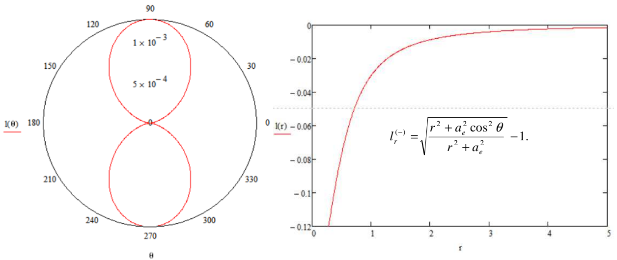
Fig. 3.1. Function graphs (3.6) for r = 10 , a_e = 0.5 , \theta = 10
