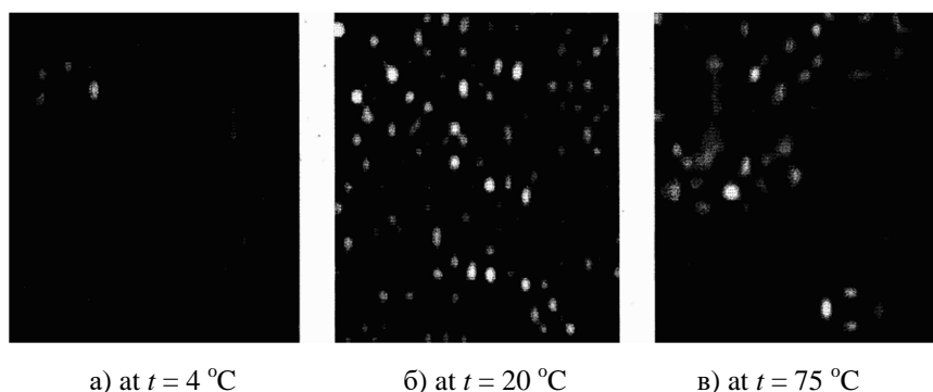
Fig. 5.2. Cluster structure of water. The typical size of the water cluster \sim 5 \cdot 10^{-6} cm Photo submitted by A. N. Smirnov
