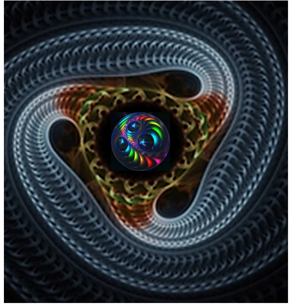
Fig. 7.1. Illustrations of the topological configuration of the outer shell and the «proton's» core
