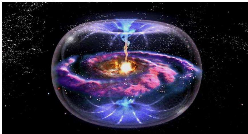
Fig. 8.3. Illustration of the toroidal-helical field of vacuum induction (i.e., magnetic field) induced around a moving and rotating galaxy https://ic.pics.livejournal.com )
