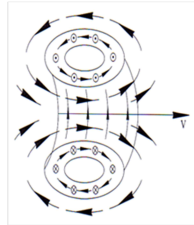
Fig. 1.2. Toroidal-helical vortex of the a \times b -subcont without a core in its neck
