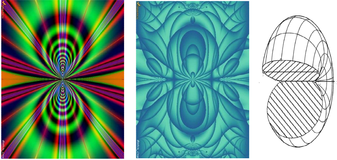
Fig. 3.4. Attempts to illustrate the distortions of the outer side of 2^3\text{-}\lambda_{m,n} -vacuum region in the vicinity of the location of the center of a stable electronic «neutrino»
