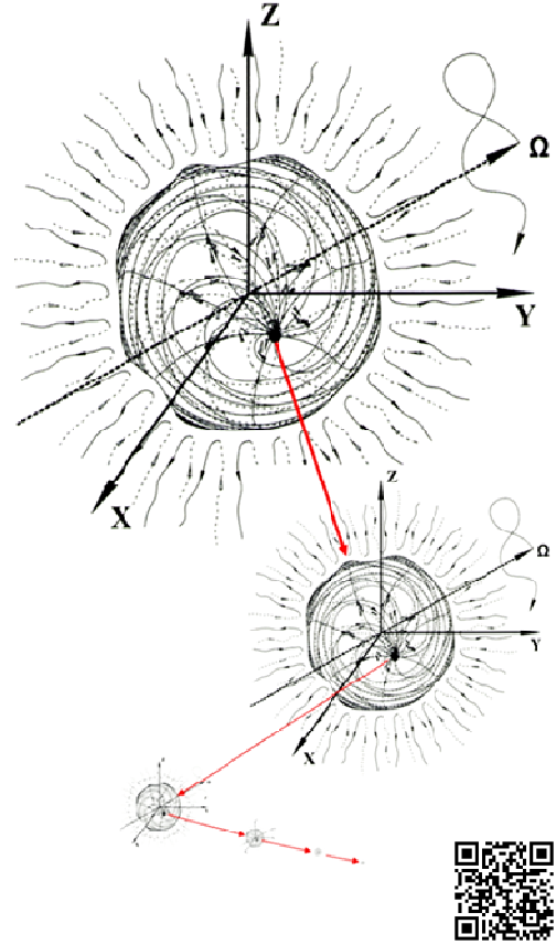
Fig. 6.2. Hierarchy of ten nested spherical vacuum formations
