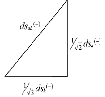
Fig. 1.3 Values of segments ds_a^{(-)} and ds_b^{(-)}
