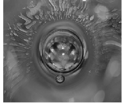
Fig. 1.1 Air bubble in liquid
