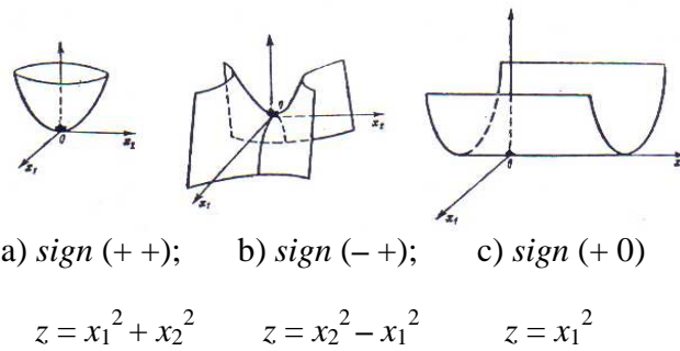
Fig. 8.1 Signature of the metric connection with the topology of 2-dimensional length (Klein 2004)
