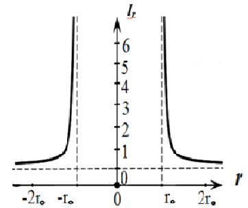
Fig. 1.2 Graph of the function l_r^{(-)} : relative length of the vacuum in the outer shell surrounding the spherical cavity. Executed in MathCad 14 for r_0 = 2
