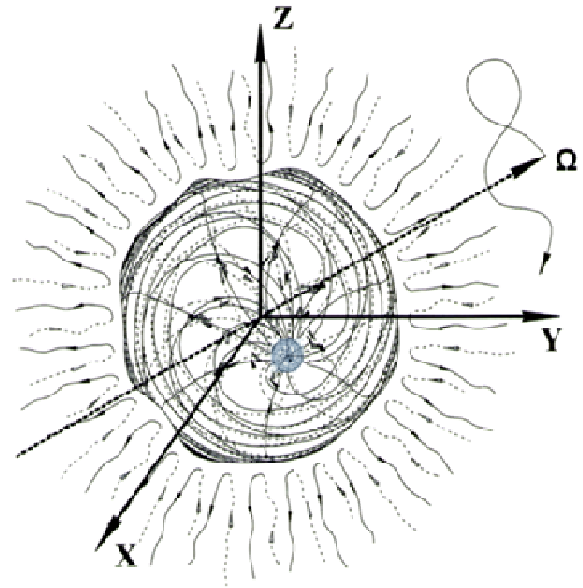
Fig. 6.1. The sequence of nested spherical vacuum formations
