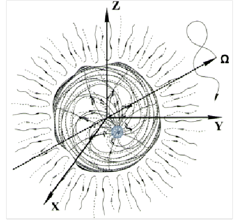
Fig. 2.2 Rotation of the core of the vacuum formation
