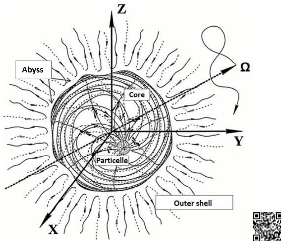
Fig. 6.3 Outer shell, abyss, core and the internal particelle of the elementary «particle»
