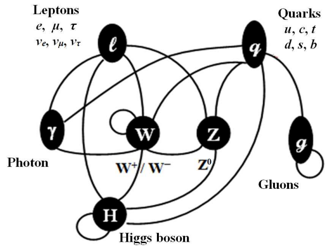
Fig 14.1 Components of the Standard Model
