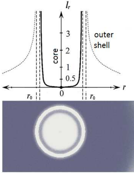
Fig. 2.1 Graph of l_r^{(-)} function - elongation of the vacuum extension in the core (i.e. within a spherical cavity)
