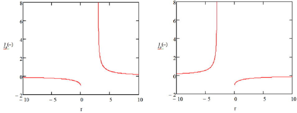
Fig.1.5. a) Graph of the function
